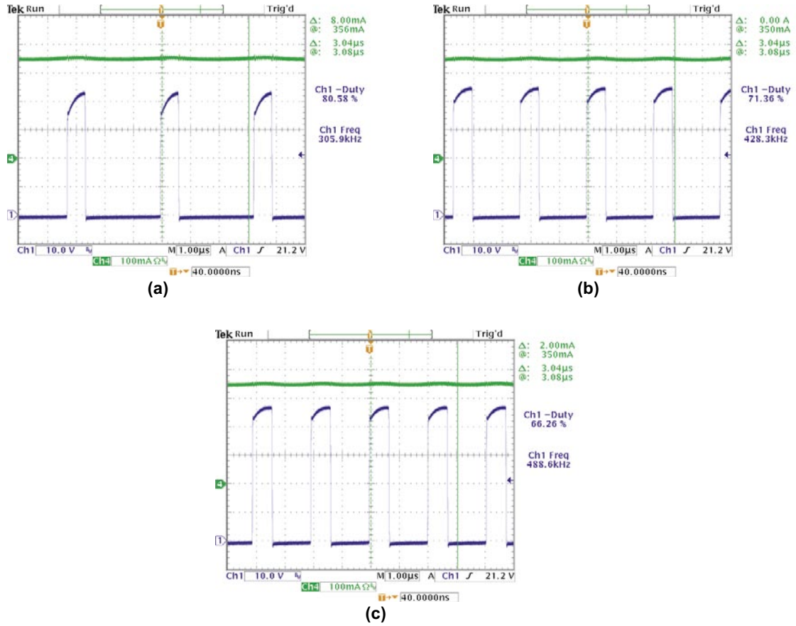
Fig. 4. Steady State Waveforms (a): 9V in; (b): 13.5V in; (c): 16V in
