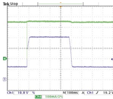
Fig. 6. LED current during step changes in the input voltage
