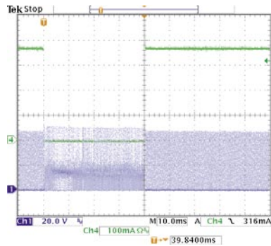
(a): Open LED Condition
